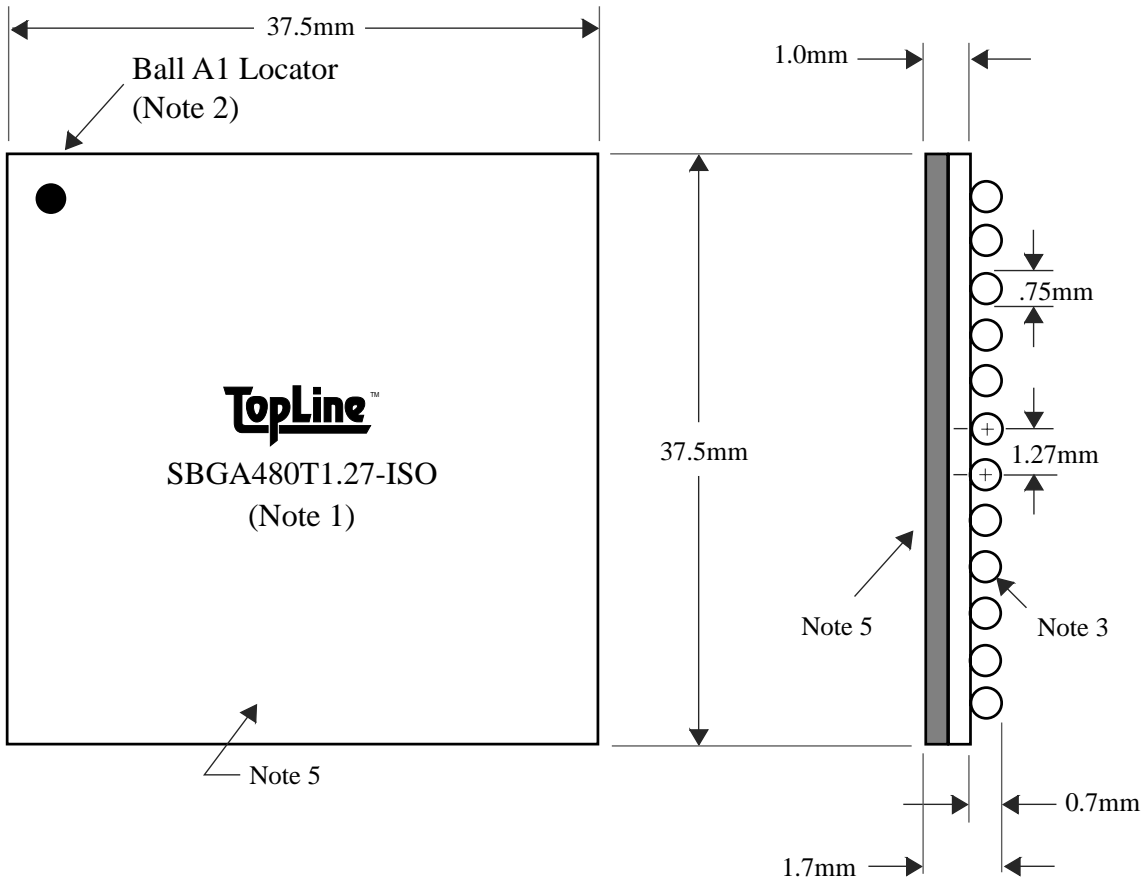
Top View
