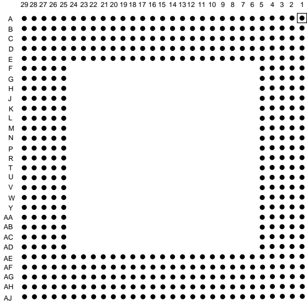
Ball View
